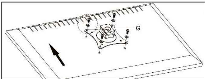
Installing the VESA Mount
