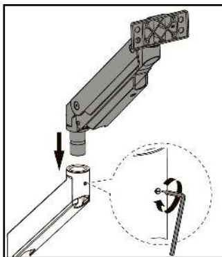
Securing the Upper Arm
