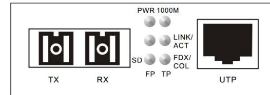
Figure 3.1 1x9 slot front panel
