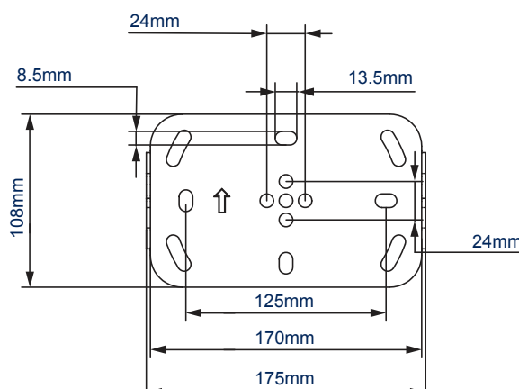
WALL PLATE - FRONT VIEW
