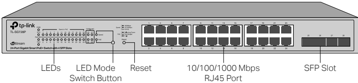
Figure 1-6 Front Panel of TL-SG728P
