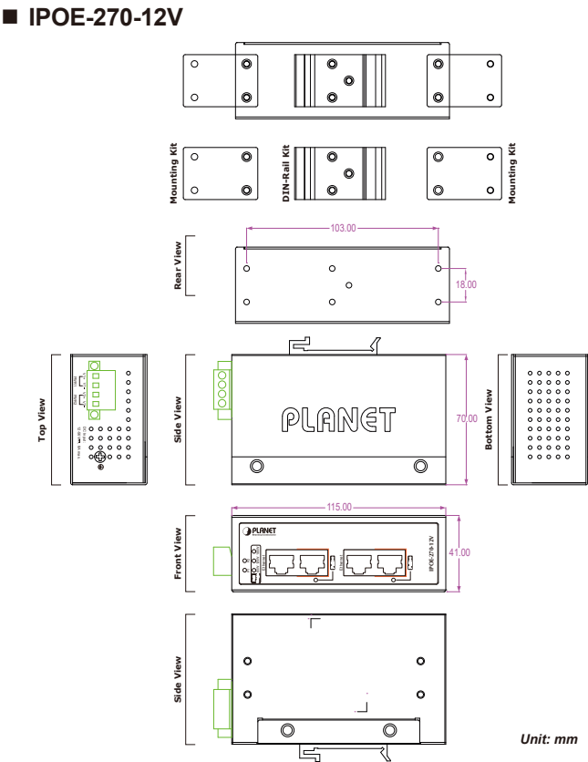
Figure 6: IPOE-270-12V Three-View Diagram
