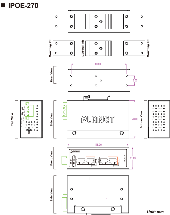
Figure 5: IPOE-270 Three-View Diagram
