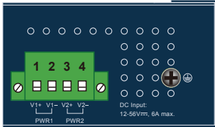
Figure 4: IPOE-270-12V Top View
