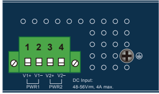
Figure 3: IPOE-270 Top View
