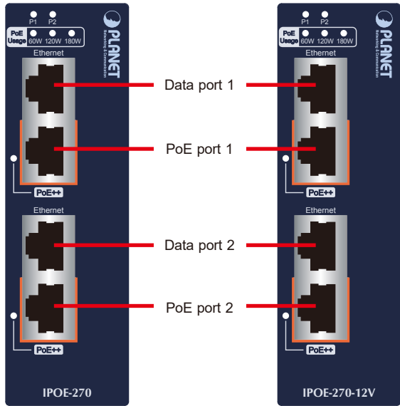
Figure 1: IPOE-270 Front View
