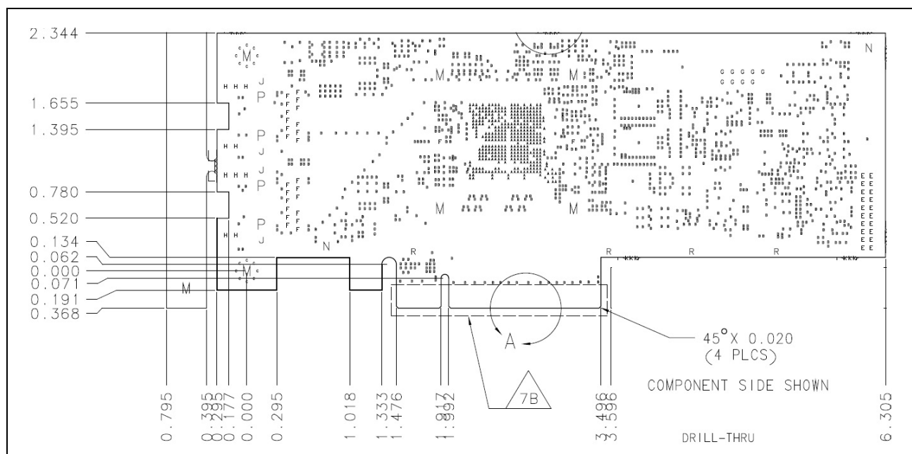
Figure 4: Board Physical Dimensions
