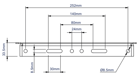
BACK VIEW
