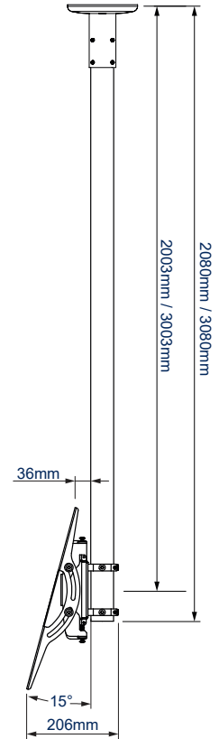
BT8424-200/300 SIDE VIEW - TILT UP
