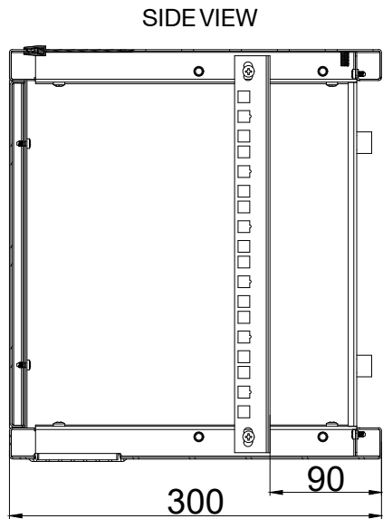
DEPTH OF WALL CABINET
