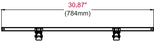
TOP VIEW EPT650
