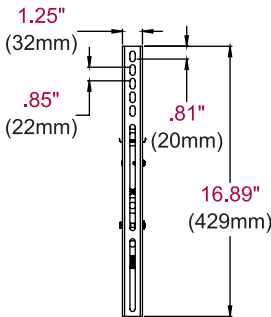
ADAPTOR DETAIL EPT650
