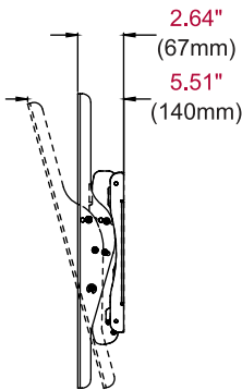
SIDE VIEW EPT650 +15°/-5° TILT
