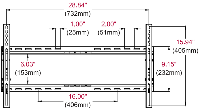
FRONT VIEW EPT650
