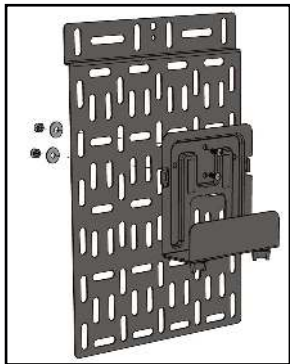
Installing the Media Device Mounting Assembly
