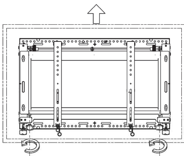
3. VERTICAL ADJUSTMENT
