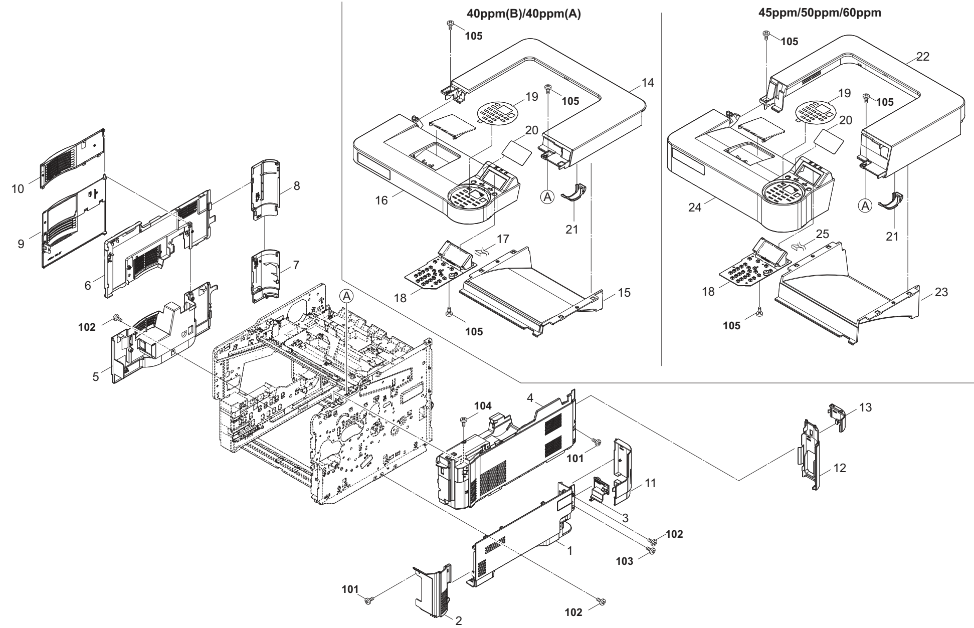
FIG. 1 Covers
