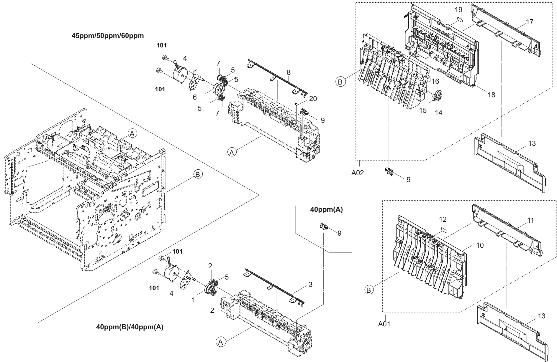
FIG. 8 Exit Section
