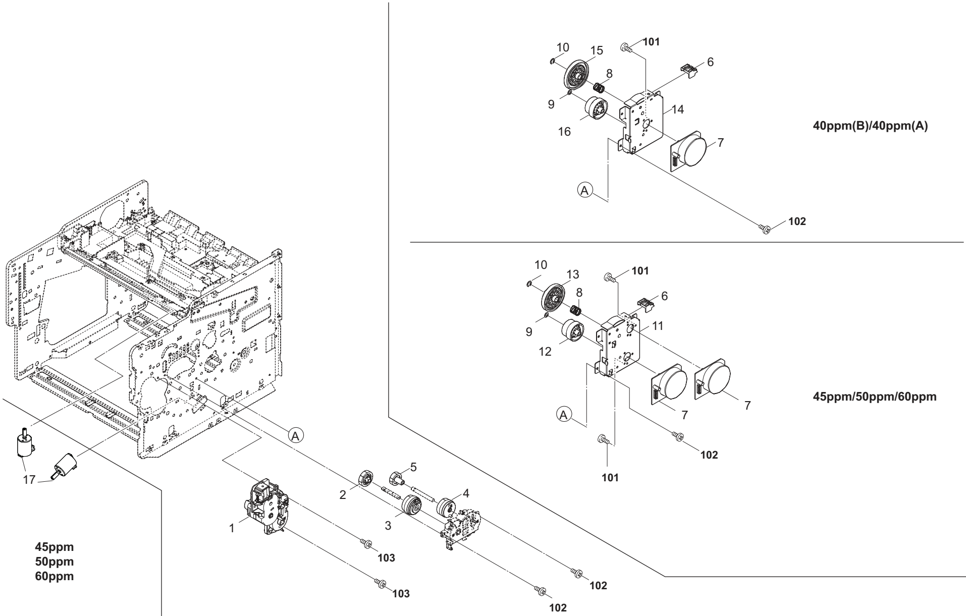
FIG. 9 Drive Section
