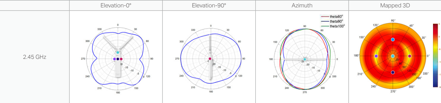
EAP110-Outdoor
