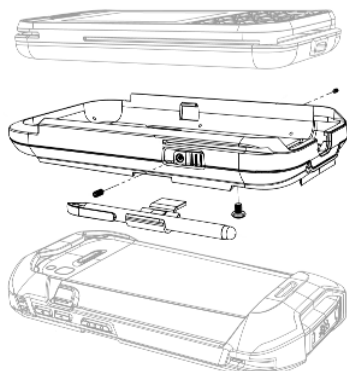
MOBILE PAYMENT SLED Part Number 367-4848 H 15.8 x W 8.2 x D 4.2cm
