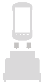
COMBINED CHARGING ADAPTER Part Number 367-4288 H 13 x W 10 x D 7.5cm
