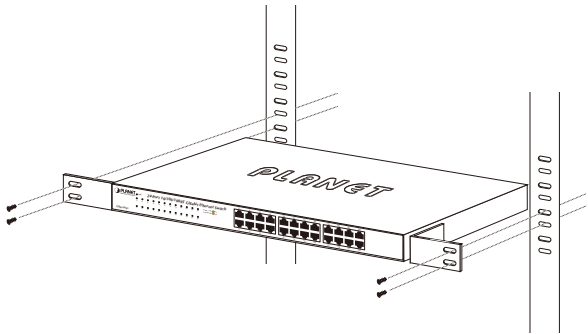
Figure 5: Mounting the Gigabit Ethernet Switch in a Rack
