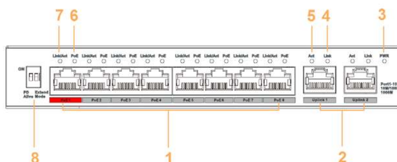
Figure 2-1 Front panel
