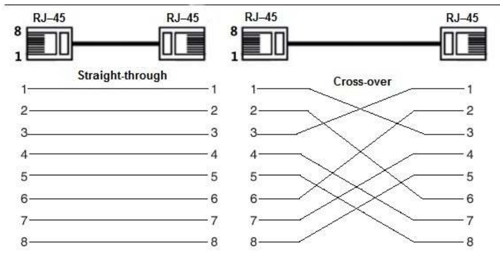
Figure 4-3 Pin description
