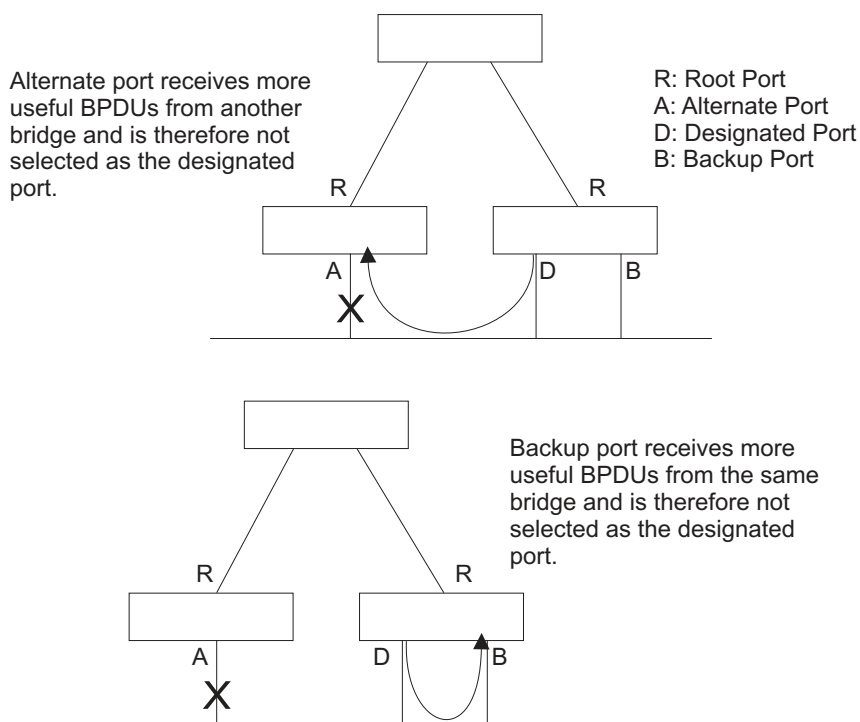
Figure 120: STA Port Roles
