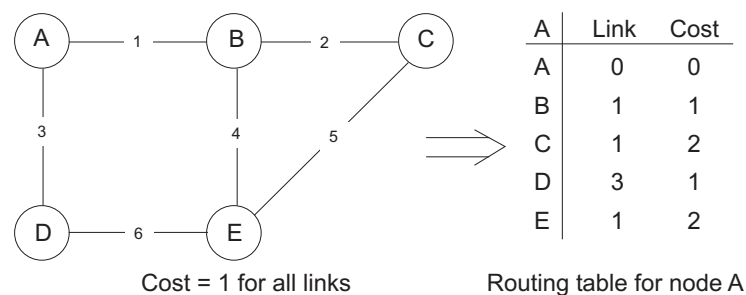
Figure 467: Configuring RIP
