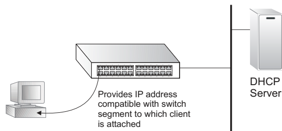
Figure 426: Layer 3 DHCP Relay Service
