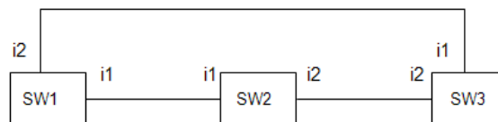
Figure 118: Determining the Root Port
