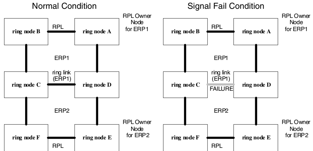
Figure 295: Ring Interconnection Architecture (Multi-ring/Ladder Network)
