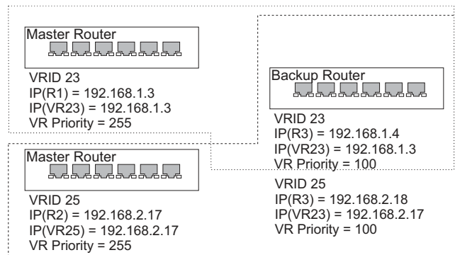
Figure 459: Several Virtual Master Routers Configured for Mutual Backup and Load Sharing
