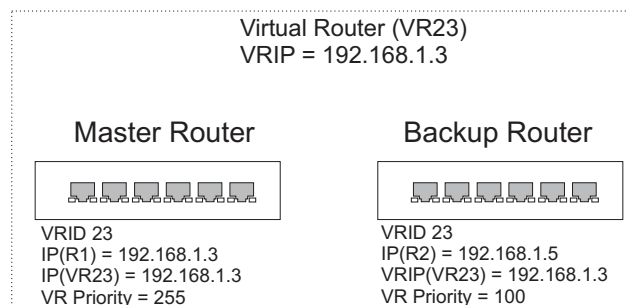
Figure 457: Master Virtual Router with Backup Routers
