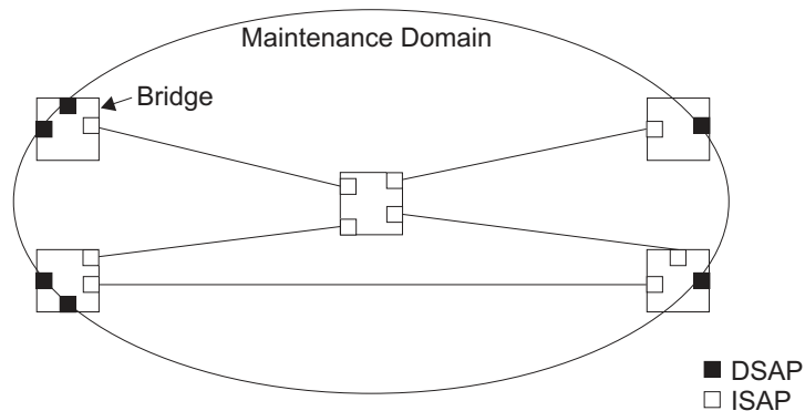
Figure 304: Single CFM Maintenance Domain
