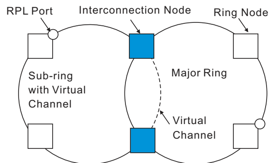
Figure 297: Sub-ring with Virtual Channel
