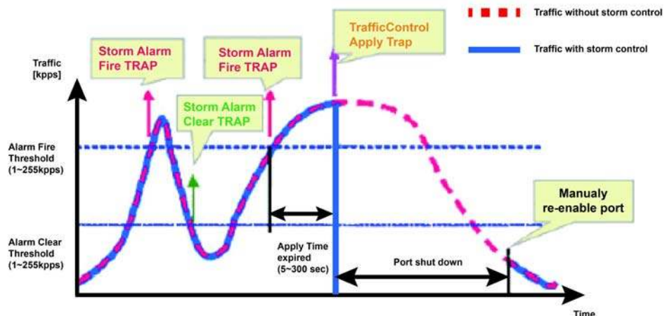
Figure 133: Storm Control by Shutting Down a Port
