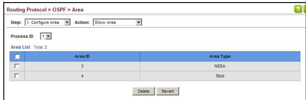
Figure 494: Showing NSSAs or Stubs
