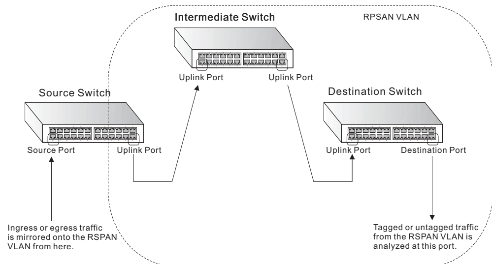
Figure 39: Configuring Remote Port Mirroring
