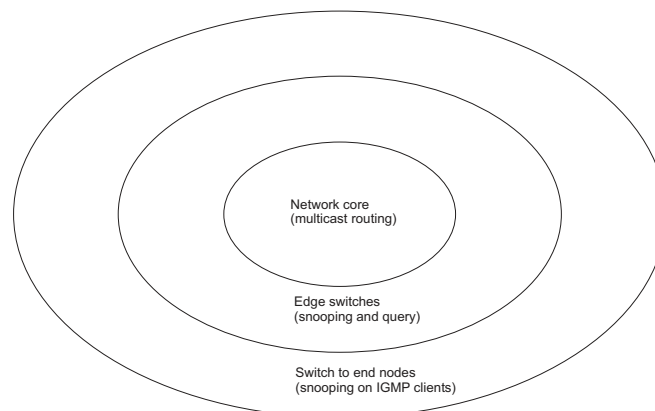
Figure 339: IGMP Protocol
