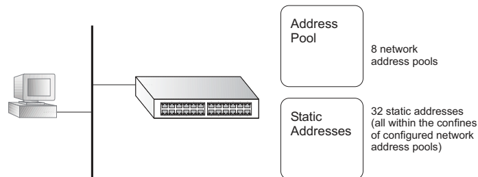
Figure 428: DHCP Server
