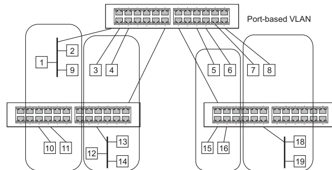
Figure 71: Using GVRP
