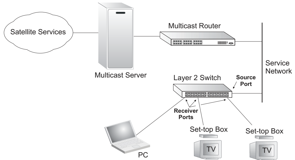
Figure 376: MVR Concept
