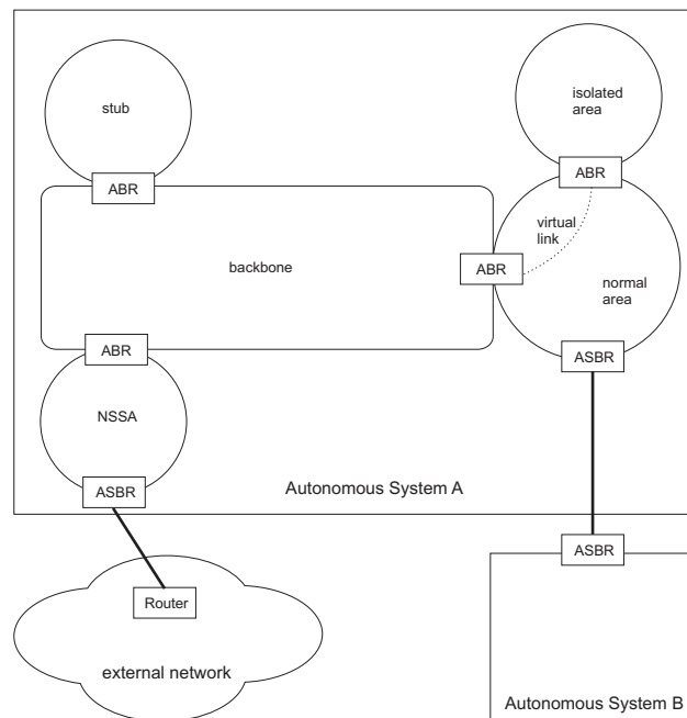
Figure 485: Configuring OSPF
