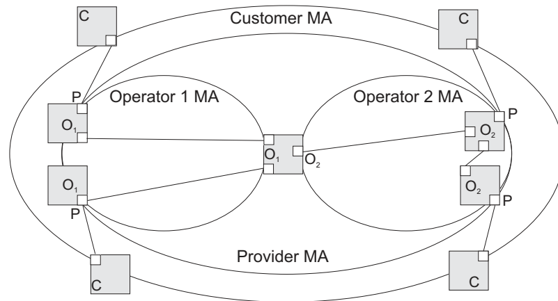
Figure 305: Multiple CFM Maintenance Domains
