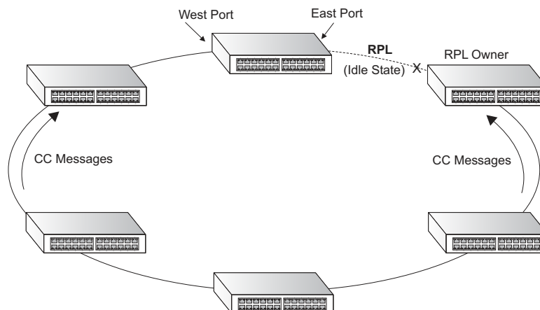
Figure 294: ERPS Ring Components
