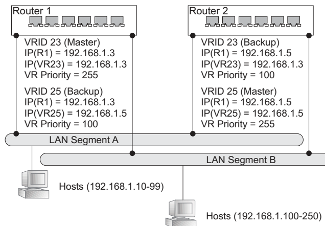
Figure 459: Several Virtual Master Routers Configured for Mutual Backup and Load Sharing
