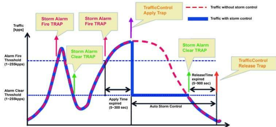
Figure 132: Storm Control by Limiting the Traffic Rate
