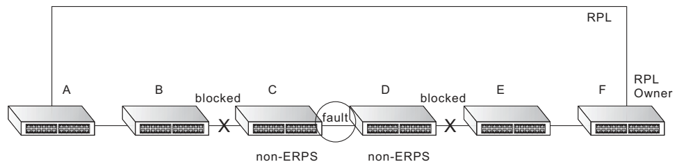
Figure 299: Non-ERPS Device Protection
