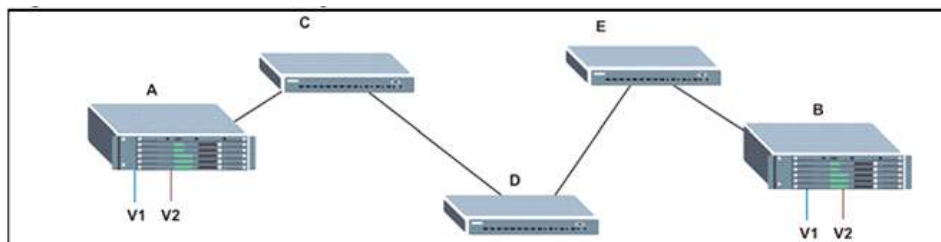
Figure 68: Configuring VLAN Trunking
