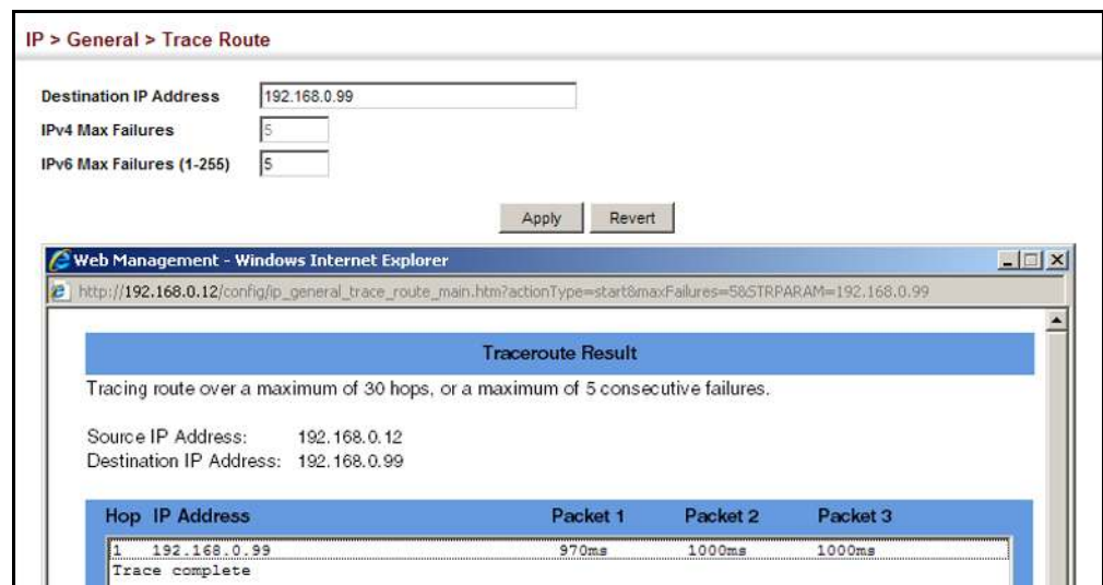
Figure 446: Tracing the Route to a Network Device
