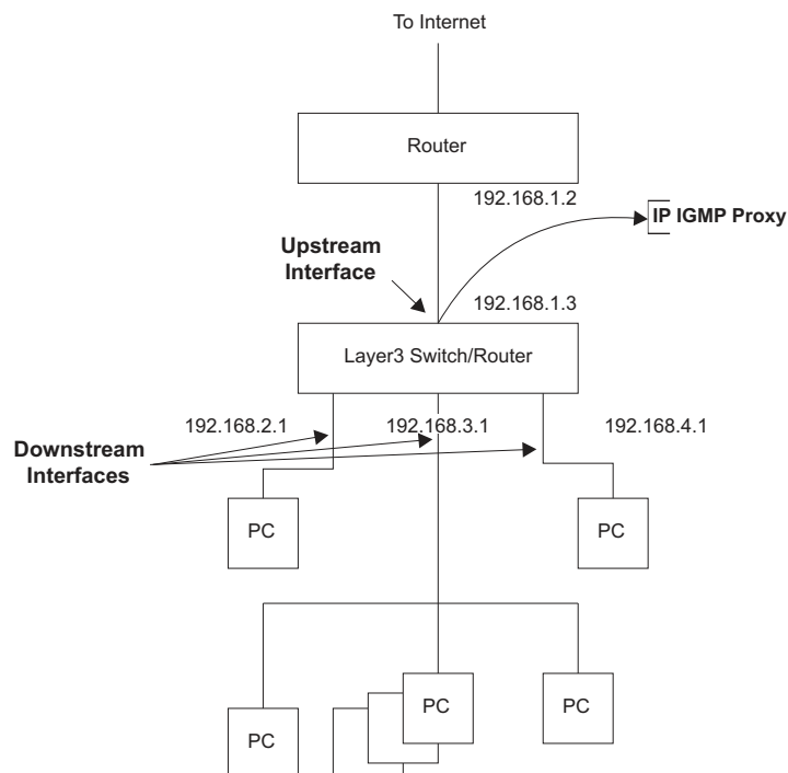
Figure 369: IGMP Proxy Routing
