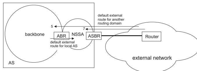
Figure 495: OSPF NSSA
