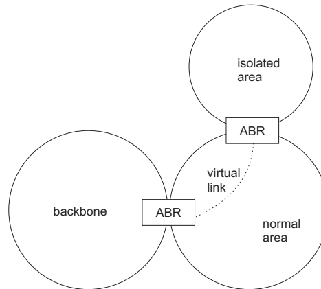
Figure 512: OSPF Virtual Link
