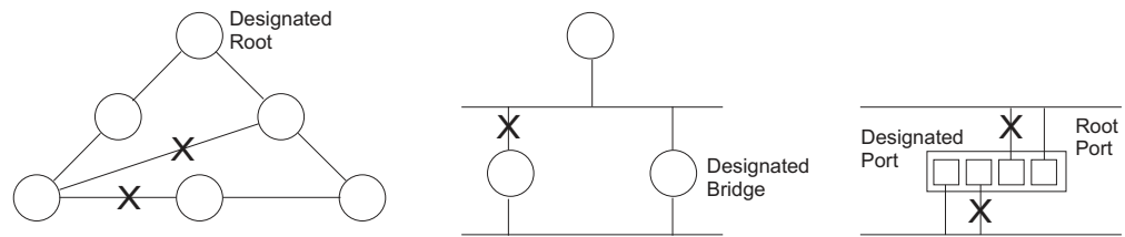
Figure 110: STP Root Ports and Designated Ports
