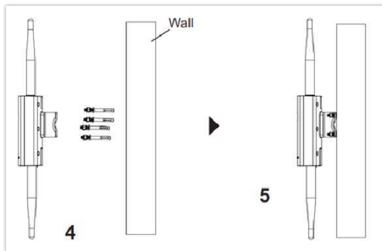
GWN7630LR/GWN7605LR/GWN7660LR Wall Mount
