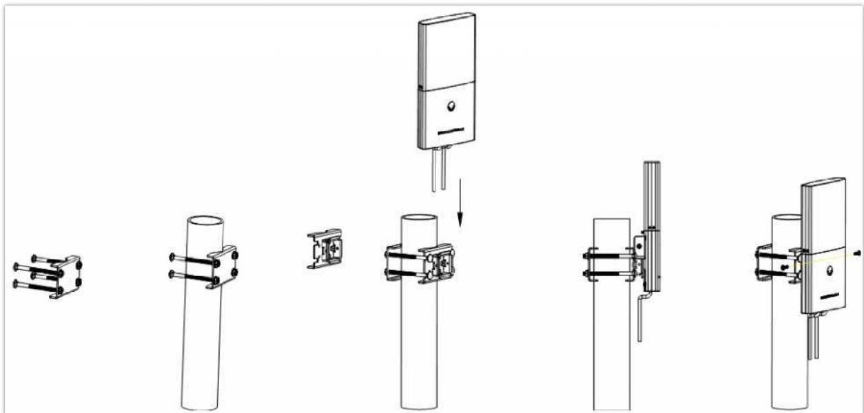
GWN7600LR Vertical Mounting
