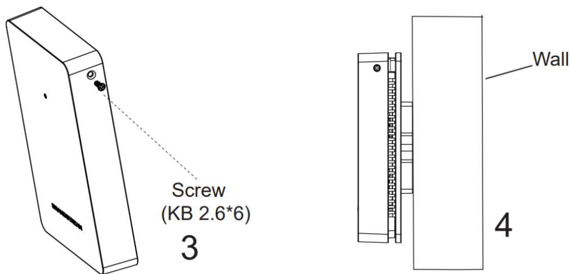
GWN7624 Wall Installation
