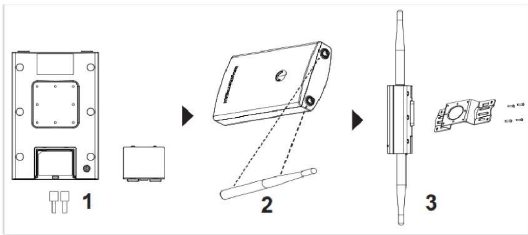
GWN7630LR/GWN7605LR/GWN7660LR /GWN7664LR Mounting Instructions
