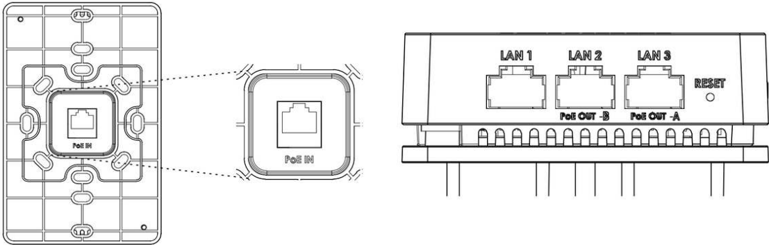
GWN7624 Ports
