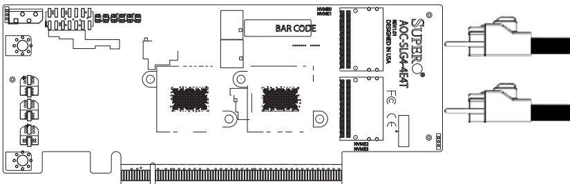
Figure 3-2. Connecting the Cables
