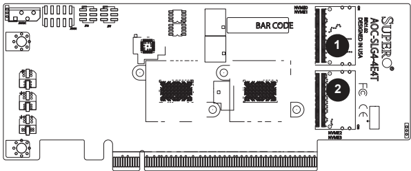
Figure 2-2. AOC-SLG4-4E4T Layout
