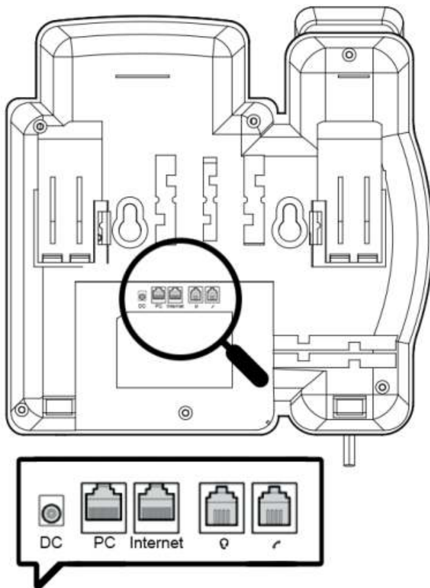
Figure 2-2: Rear View
