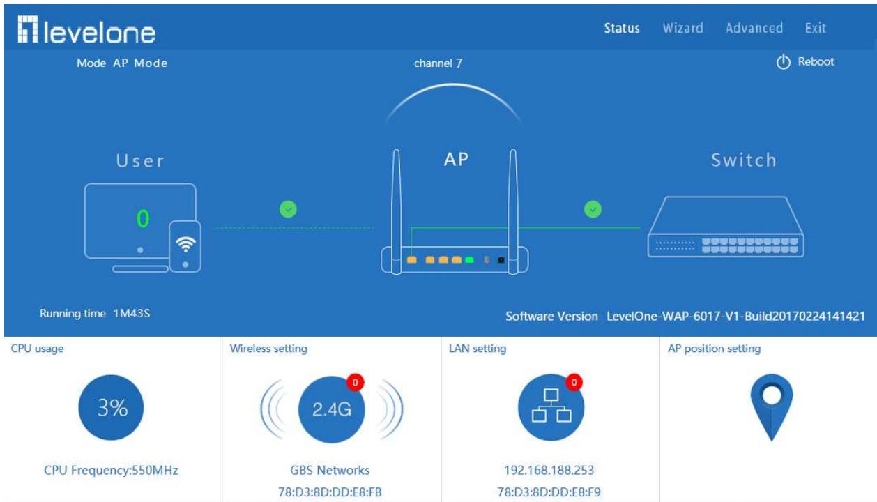
P35 Status in AP Mode
