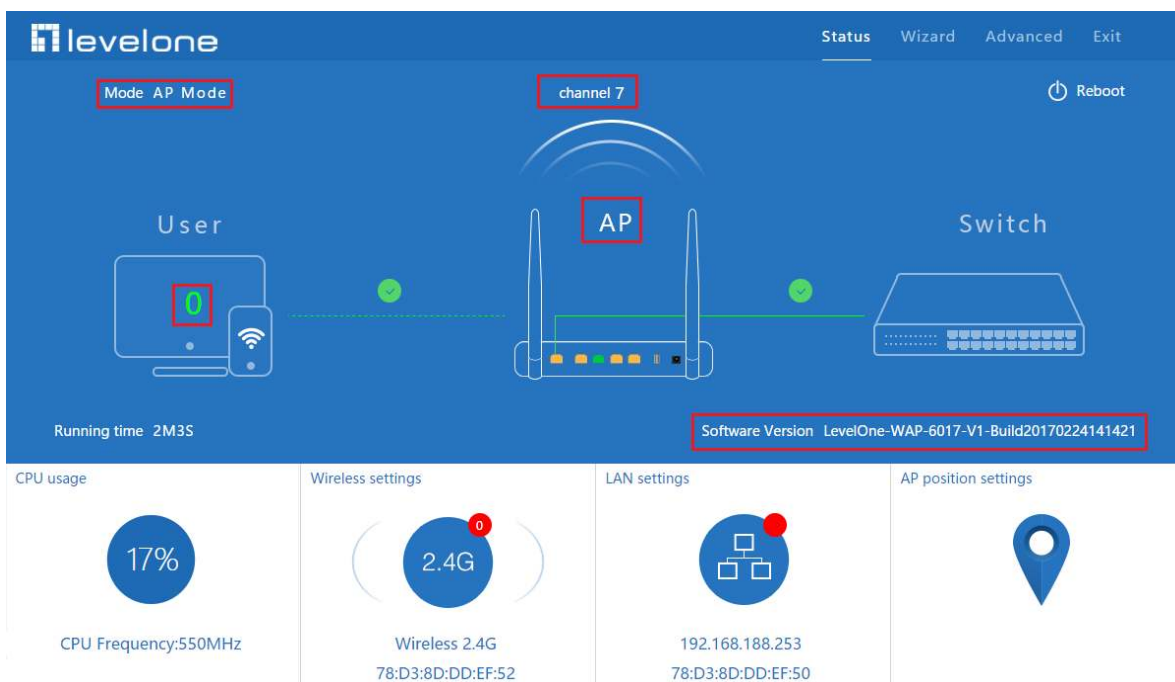
P12: WAP-6017 Device Status
