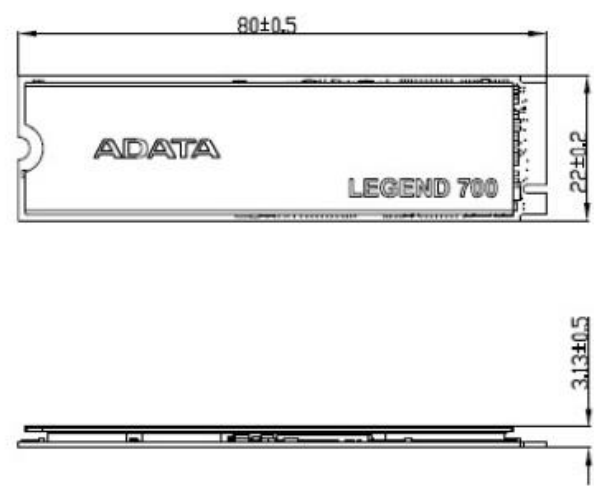
<With heatsink>
