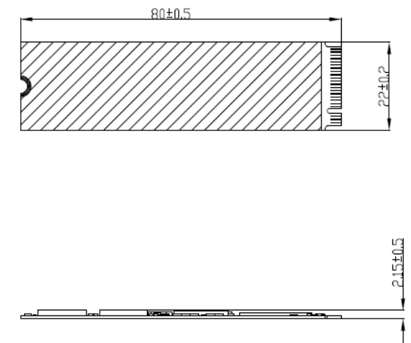
<Without heatsink>
