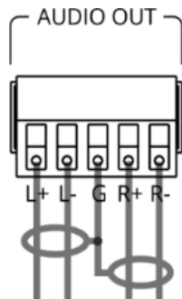
Figure 4: Connecting to a Balanced Stereo Audio Acceptor
