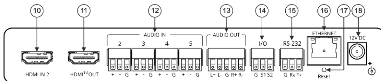
Figure 2: DSP-62-AEC Digital Sound Processor Rear Panel
