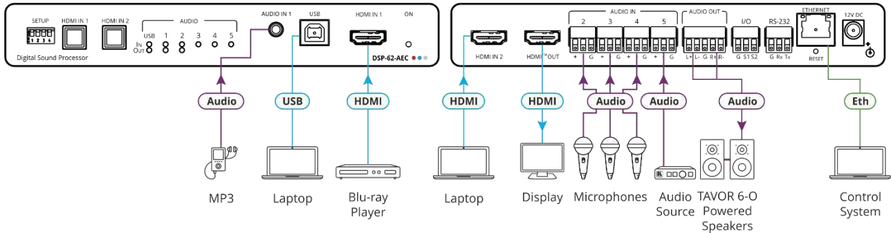
Figure 3: Connecting to the DSP-62-AEC
