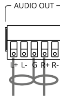
Figure 5: Connecting to an Unbalanced Stereo Audio Acceptor
