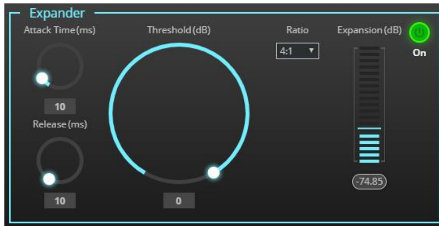
Figure 25: Processing View – Expander Module
