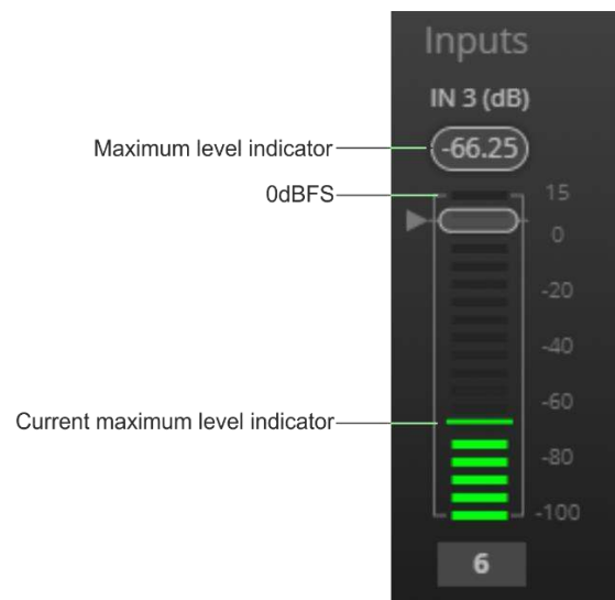
Figure 19: Level Measurement Indicators
