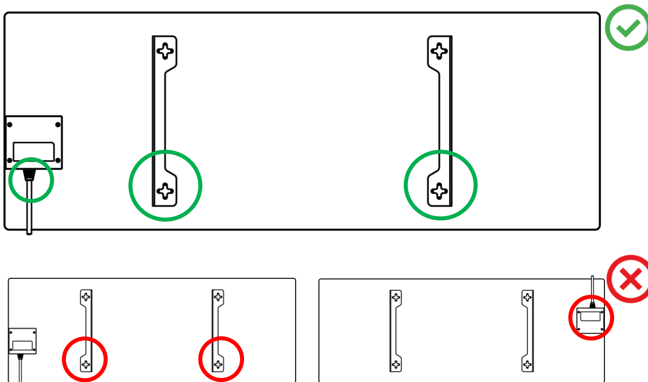
Figure 8 – Installation of the brackets
