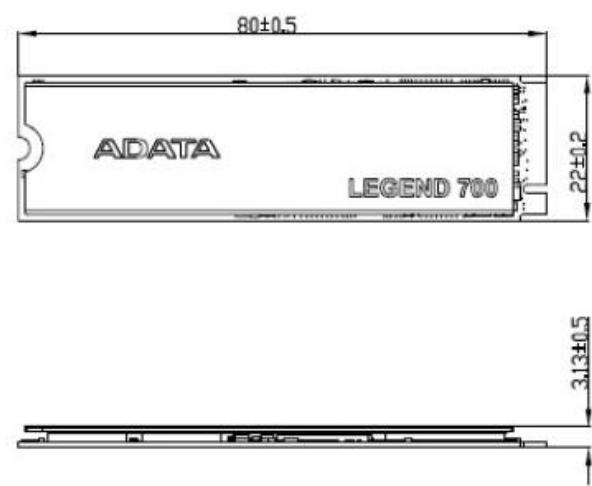
<With heatsink>
