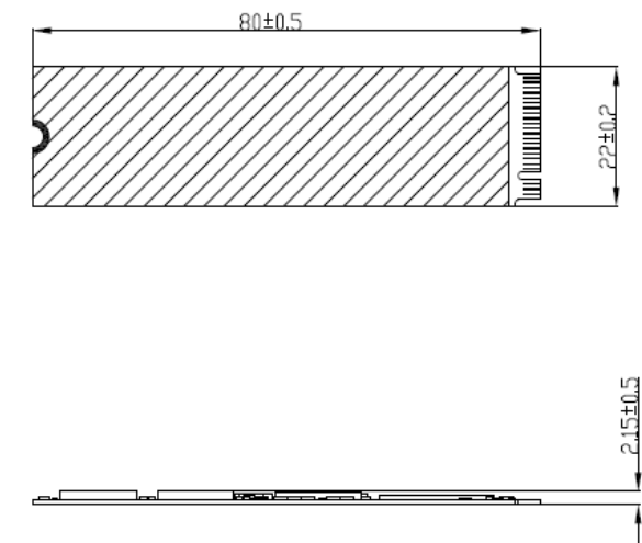
<Without heatsink>
