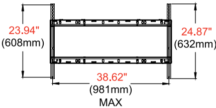
ADAPTOR BRACKET
