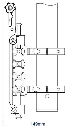
POLE MOUNTED*
