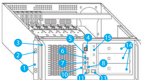
Figure 2.6.1.7 - SC01-3504-10B chassis
