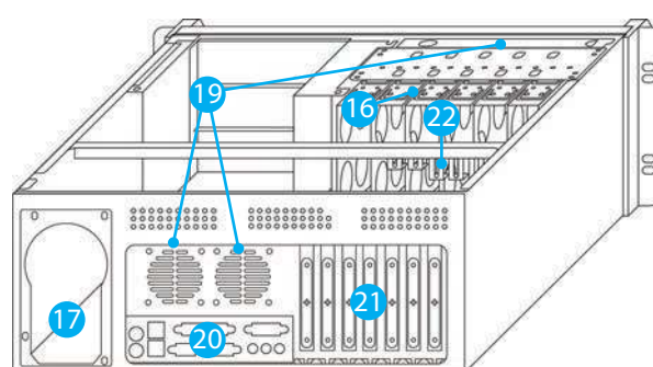
Figure 2.6.1.8 - SC01-3504-10B chassis
