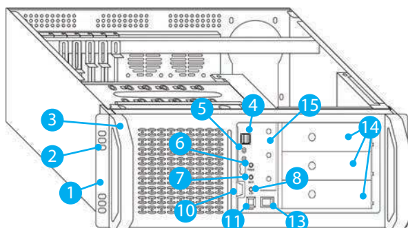
Figure 2.6.1.1 - SC01-4504-08B chassis
