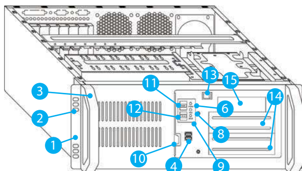
Figure 2.6.1.3 - SC01-4504-10B chassis
