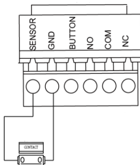
Figure 4-7 Magnetics Connection
