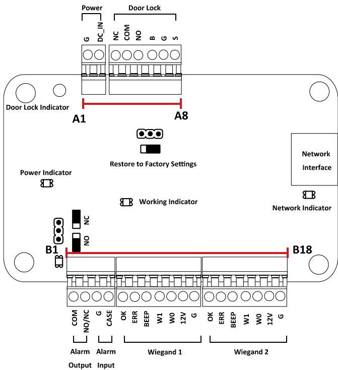
Figure 3-1 DS-K2801 Terminals
