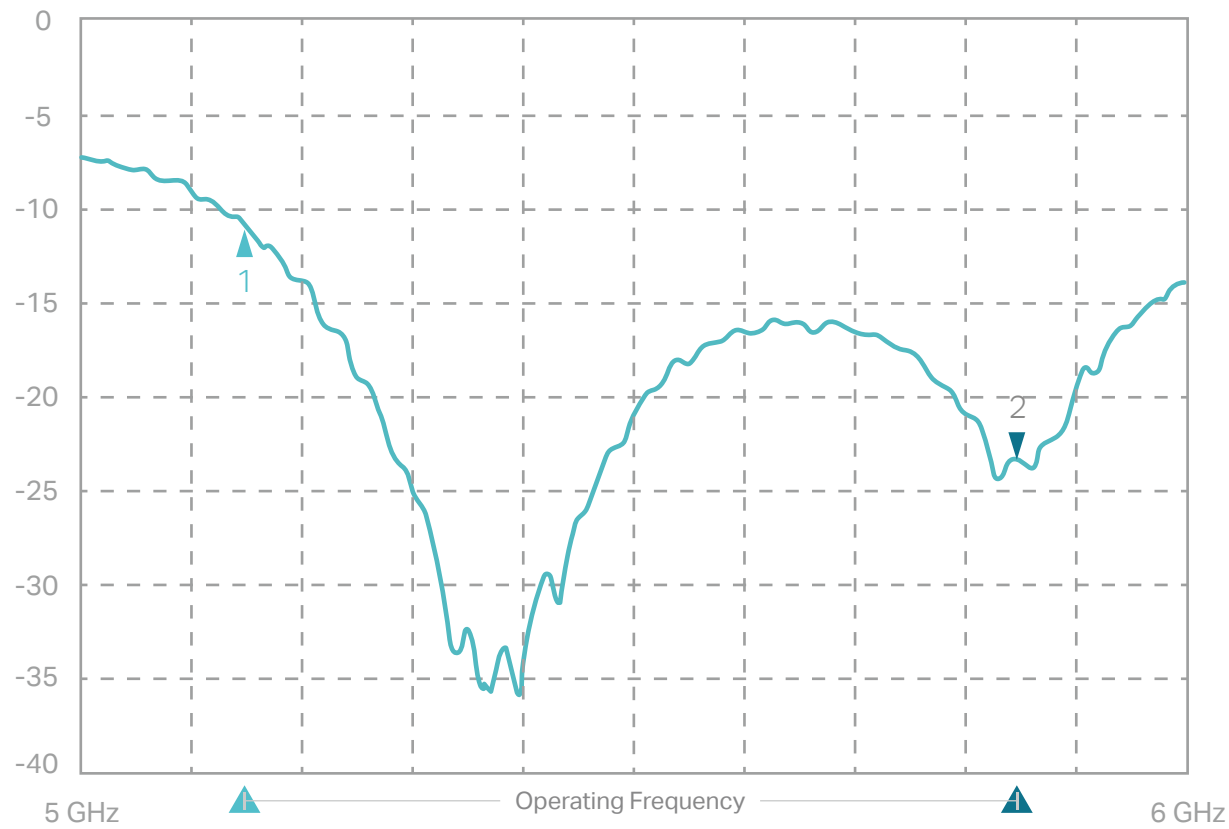
Return Loss
