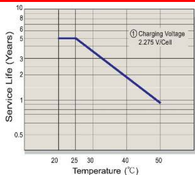
Float(or Standby) Service Life
