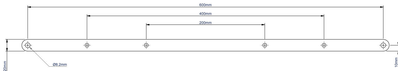
FRONT VIEW
