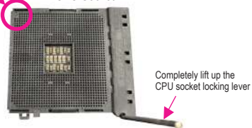
AM4 CPU Socket
