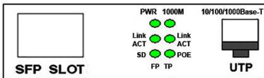
Figure 3-3: Product Outlook of DN-82140
