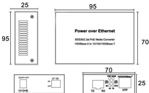
Figure 3-1: Product Outlook of DN-82140
