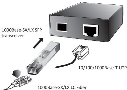
Figure 5-2: DN-82140 Installation
